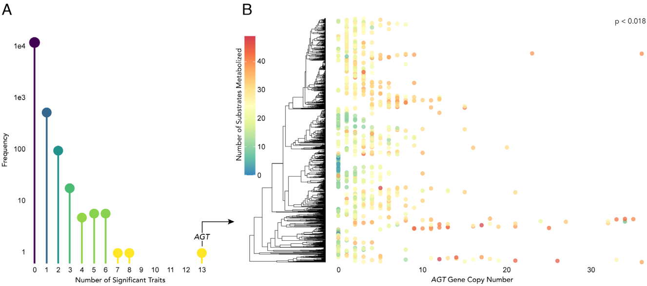
Fig. 3. Keystone gene families influence innovation of multiple metabolic traits. (A) Histogram of the number of traits significantly associated with each of 14,785 gene families. Of the 739 families with a significant relationship, most (81%) are associated with just one trait, with the remaining 19% associated with two or more traits. Furthermore, a minority of keystone families show significant effects on several ( \geq 4 ) traits. (B) An extreme example of a keystone gene family encoding AGT . Size of the AGT gene family mapped onto a species phylogeny, colored by the total number of substrates metabolized by each species. On average, the AGT gene family is significantly ( P < 0.018 ) larger in generalist species than in specialist species.
