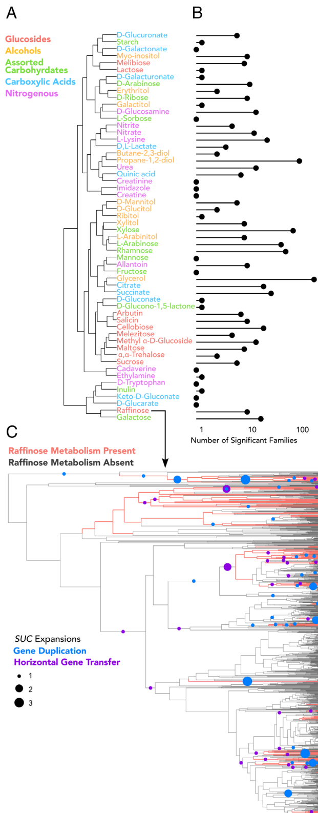
Fig. 2. Gene family expansion and contraction was significantly linked to trait gain and loss in 80% of metabolic traits. (A) All 56 metabolic traits examined by this study, clustered by gene family affinity. Traits are clustered by z-scores across families; closer traits share more similar correlations with the same gene families. (B) Number of gene families that are significantly associated with each metabolic trait. (C) Example of a convergent trait (raffinose metabolism), driven by convergent expansions within the same gene family ( SUC ). The presence of raffinose metabolism is denoted by the red branches and its absence by the black branches. Note that the presence of raffinose metabolism (in red) coincides with gene duplication (blue dots) and horizontal gene transfer (purple dots) events of the SUC gene family across the yeast species phylogeny.
