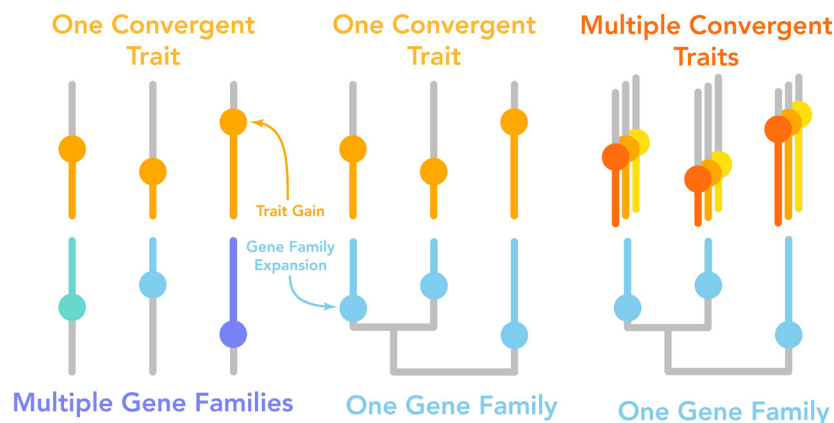
Fig. 1. Models of convergent evolution. Gains of novel traits ( Top ) and genes ( Bottom ) are represented by colored dots which appear across lineages (lines), with unique traits/genes represented by separate colors. Top row: convergence occurs when the same trait appears multiple times across separate lineages on the tree of life. Bottom row: convergent traits can originate in a homologous fashion by changes within a single gene family ( Center ), as is the case with image-forming eyes, or in an analogous fashion by changes across multiple different gene families ( Left ), as with freezing resistance. Likewise, gene family evolution may cause convergence in one trait ( Center ) or many different traits ( Right ). Our study reports that homologous events in gene family evolution explain convergence in 80% of analyzed traits ( Center ). While the majority of these families are associated with a single trait ( Center ), we also find evidence of select few “keystone” gene families that exhibit pleiotropic effects across many different traits ( Right ).
